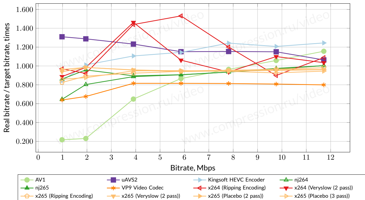
Figure 6: Bitrate handling—use case “Ripping Encoding,” Infinif sequence.
