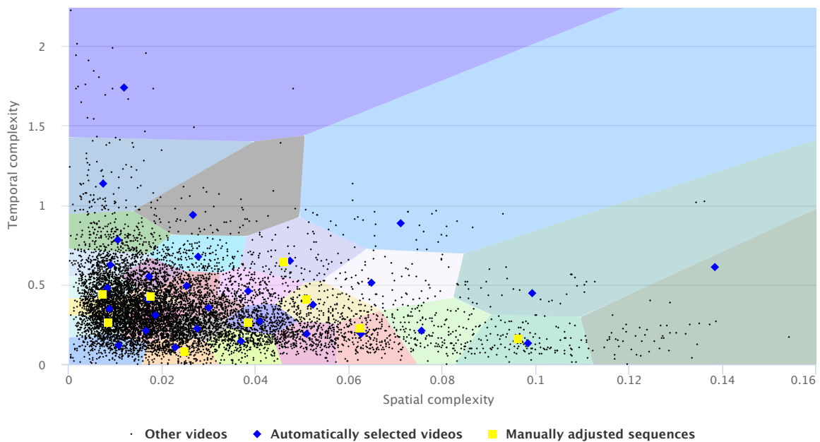
Figure 49: Adjustments to test dataset
