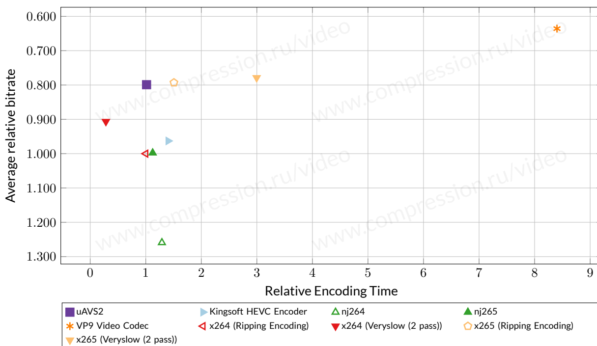
Figure 11: Speed/quality trade-off—use case “Ripping Encoding,” Infinit sequence, YUV-SSIM metric.
