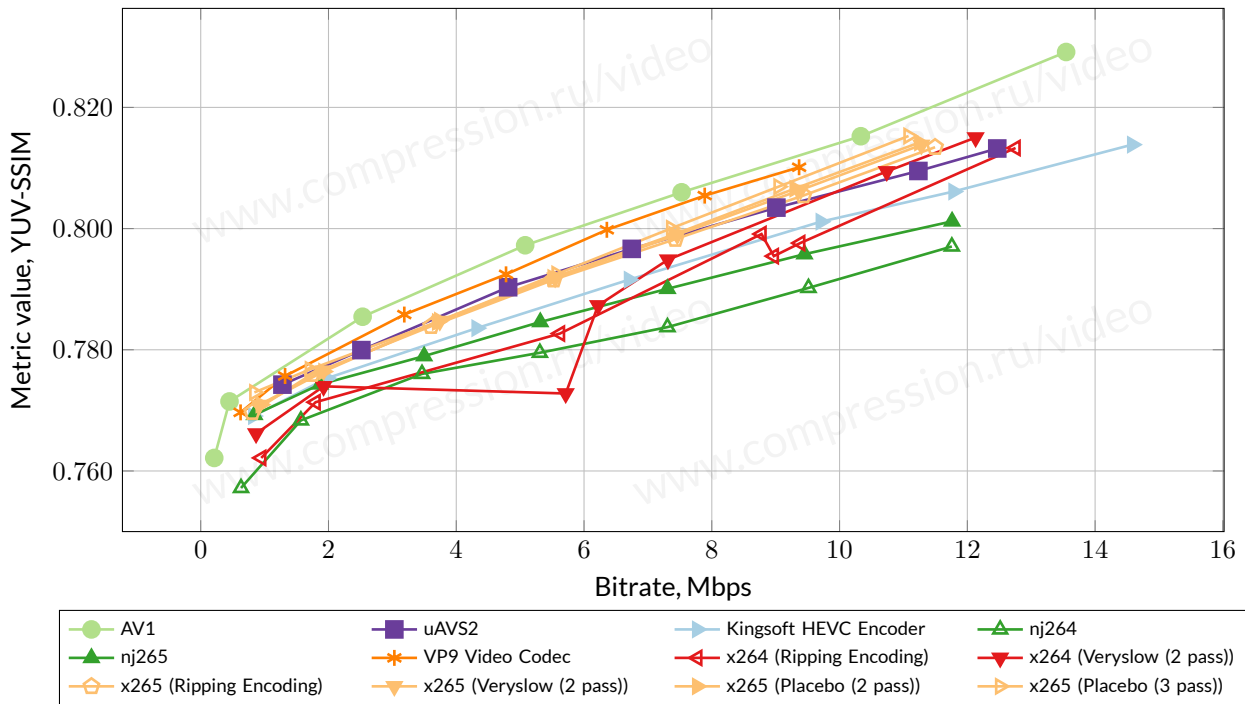
Figure 2: Bitrate/quality—use case “Ripping Encoding,” Infinet sequence, YUV-SSIM metric.
