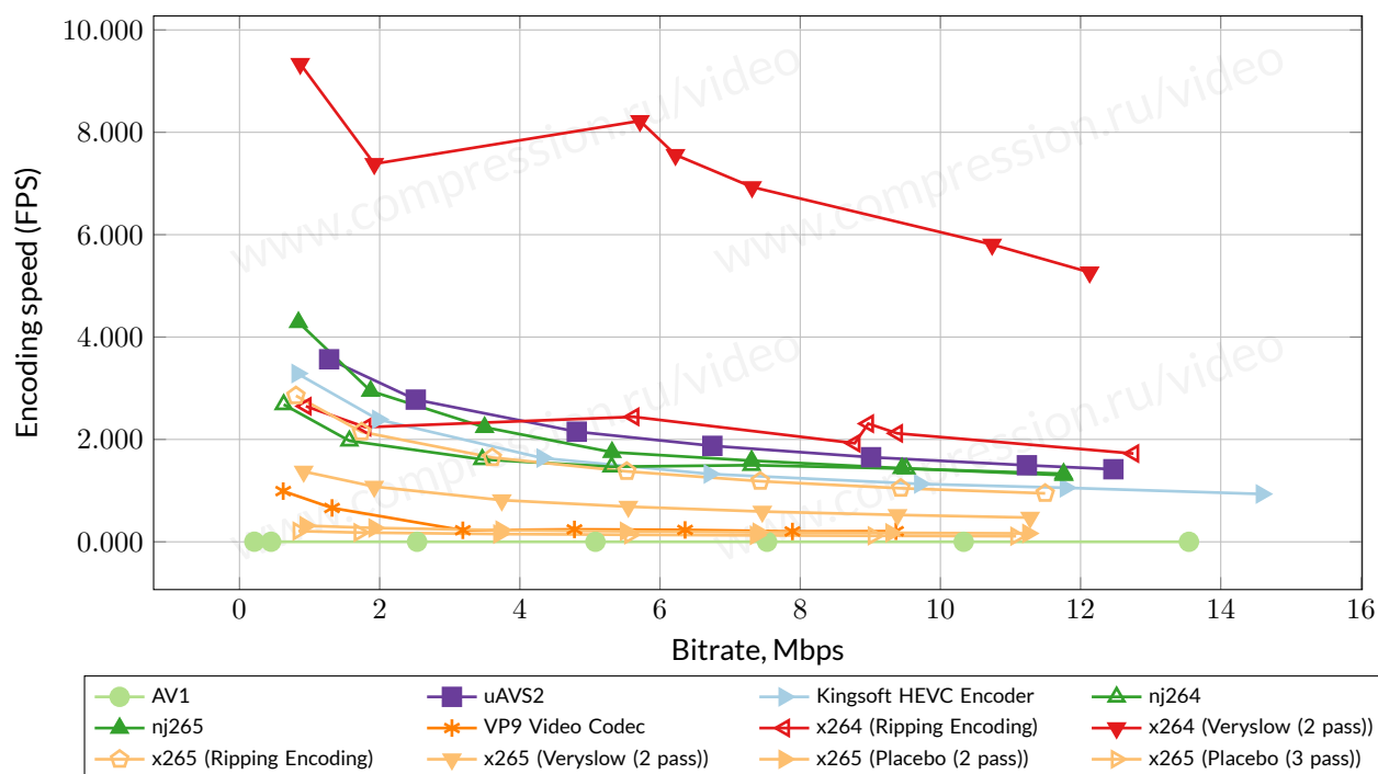
Figure 4: Encoding speed—use case “Ripping Encoding,” Infinet sequence.
